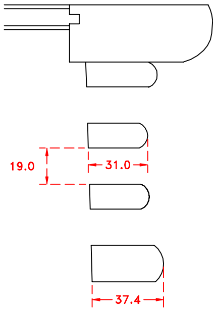
Half size Detail: Front section.
