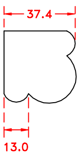
Half size detail: Leg section.
